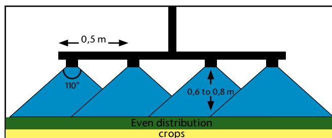
Boom height correctly adjusted
